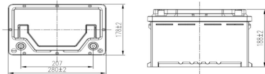
2 Dimension drawing
