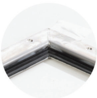
Replaceable double-lip EPDM gasket
